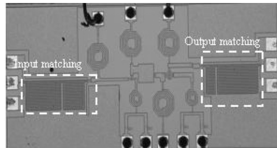
Fig. 6 Microphotograph of PA with the proposed impedance-matching circuits fabricated in TSMC 0.35\mu\text{m} SiGe BiCMOS one poly three metal process. (Chip size: 2.38\text{ mm} \times 1.05\text{ mm} ).
